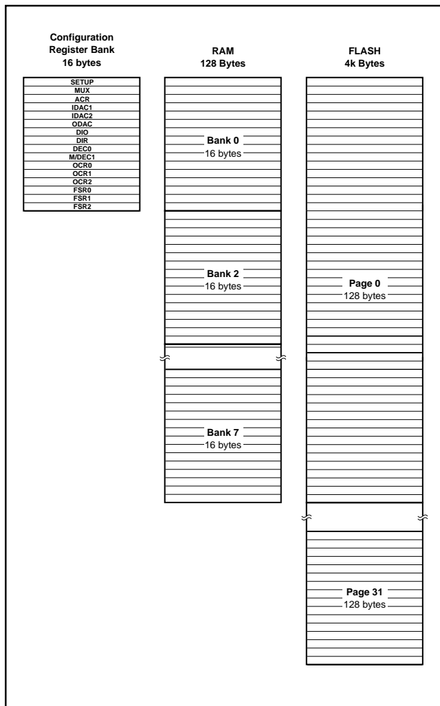
FIGURE 5. Memory Organization.
