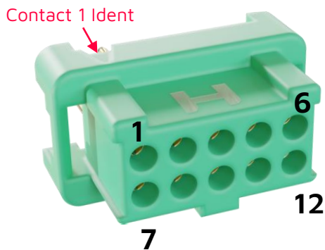
Female PCB mounted
