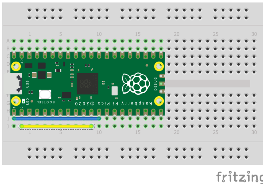
Figure 12. Wiring two of the Pico's ports together. Be sure to wire UART0 TX to UART1 RX and UART0 RX to UART1 TX.
