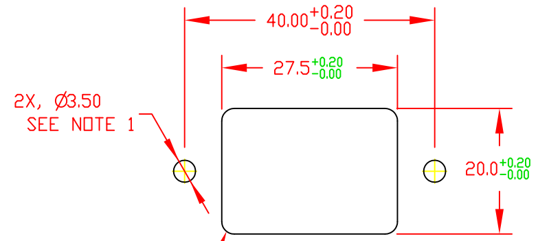
PANEL CUTOUT FRONT SIDE MOUNTING
