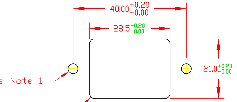
PANEL CUTOUT REAR SIDE MOUNTING
