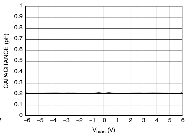
Figure 10. CV Characteristics
