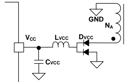
Figure 5: Forward Mode V_{CC} from N_A Winding
