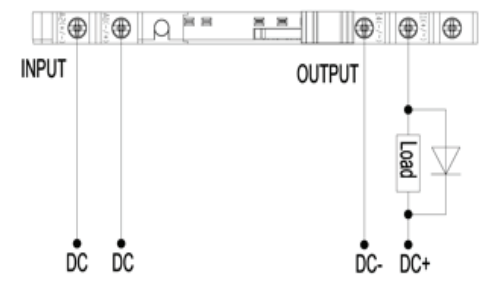
ASR-SMD...D...-P/R/S/TK Series
