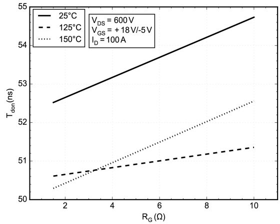
Figure 14. Typical Turn-On Switching T_{d(on)} vs. R_G
