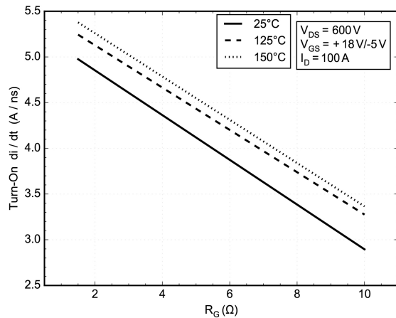
Figure 22. di/dt ON vs. R_G
