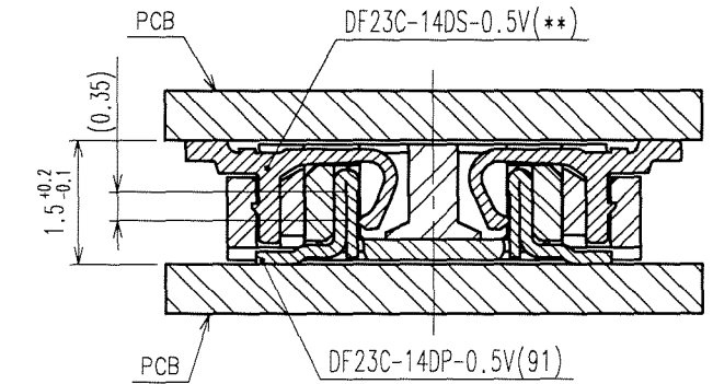
Fig.4 : MATING VIEW
