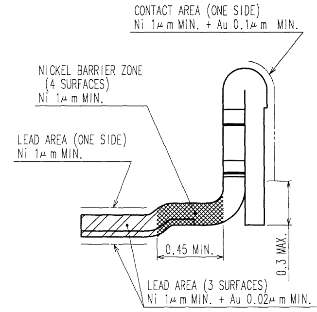
Fig.2 : PLATING SPECIFICATION (40:1)
