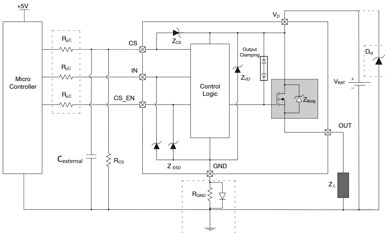
Figure 33. Application Schematic
