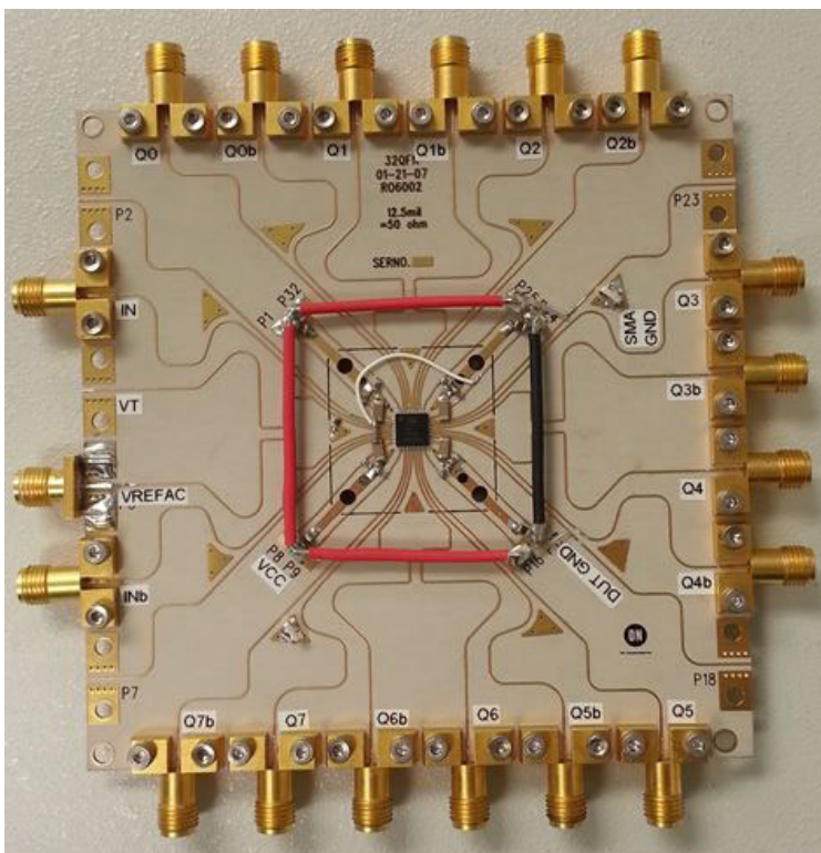
Figure 1. Test Board
