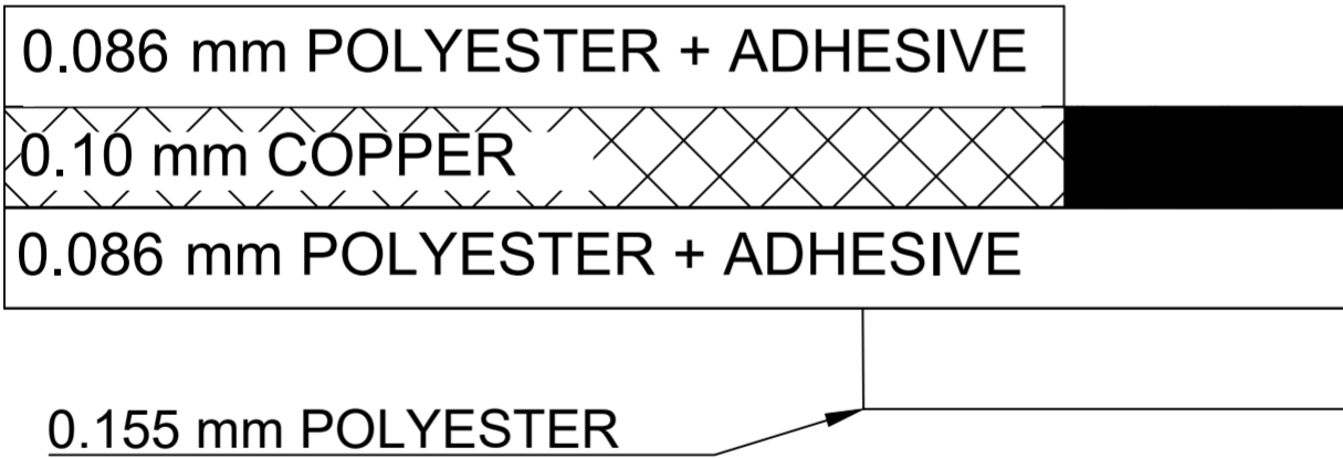
CROSS-SECTION
