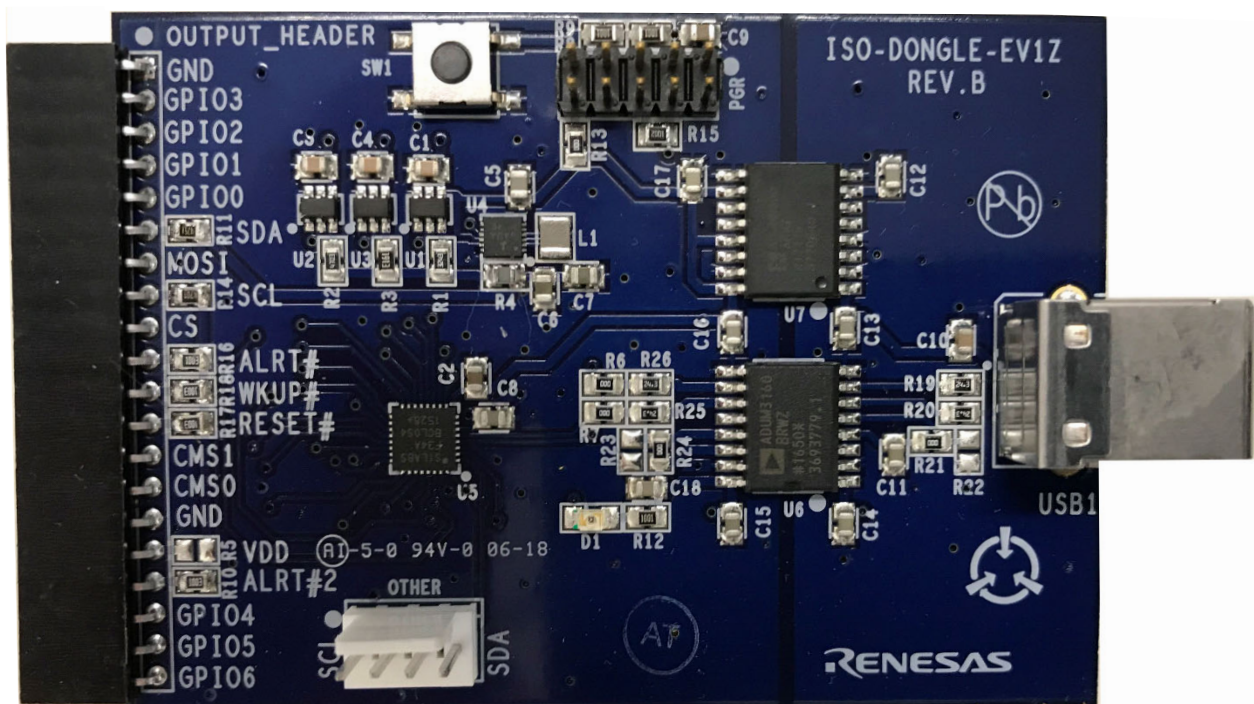
Figure 6. ISO-DONGLE-EV1Z Communications Dongle
