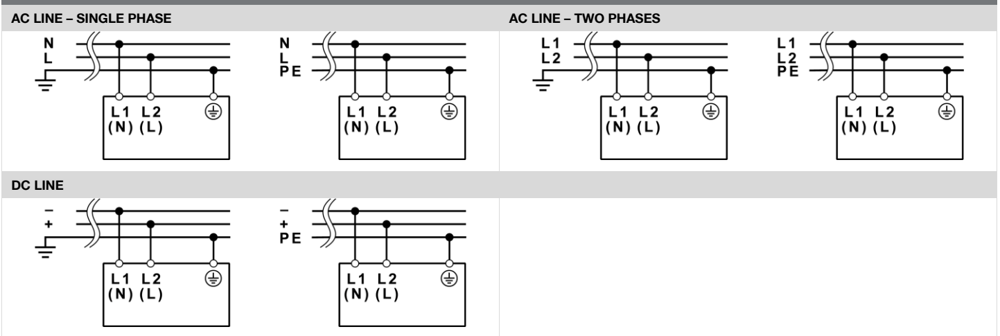
FIG.7 - INPUT CONNECTIONS
