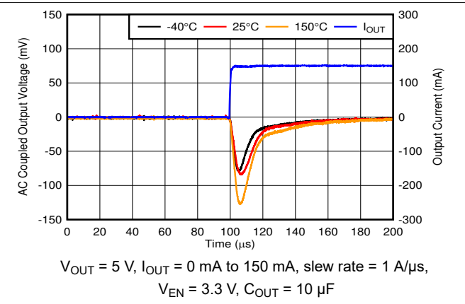
Figure 6-22. Load Transient, No Load to 150-mA Rising Edge
