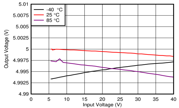
Figure 6-4. Line Regulation vs V_{IN}
