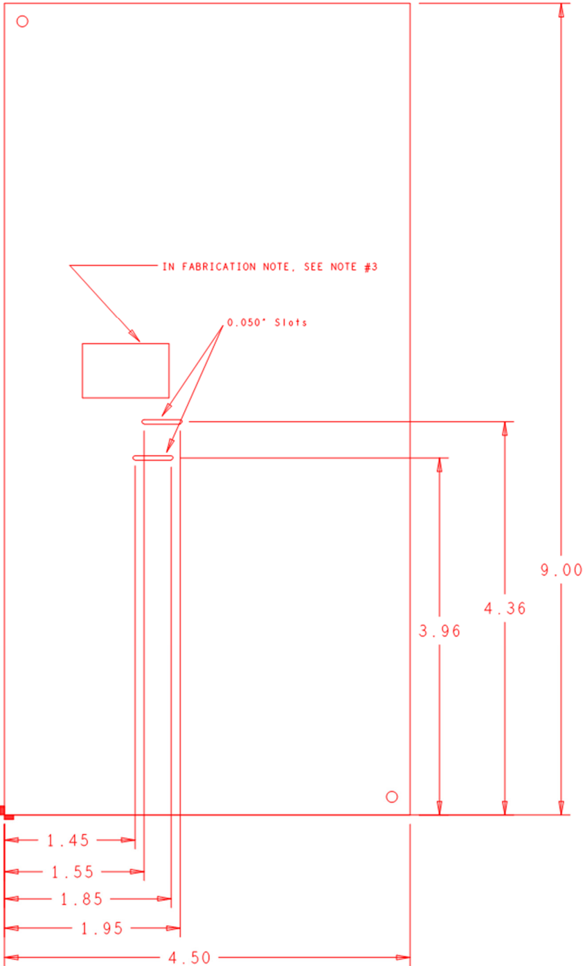
FIGURE 7 Circuit Outline
