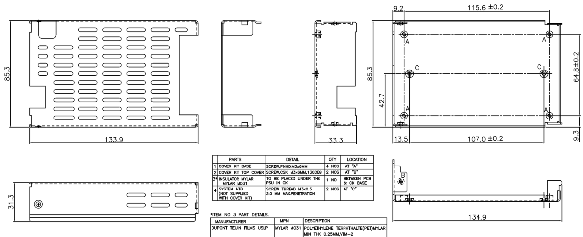
WLP350-CK. MECHANICAL OUTLINE DIMENSIONS.
