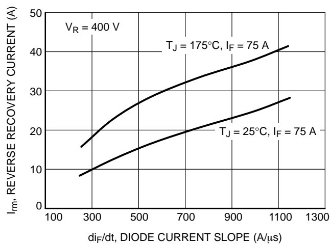
Figure 22. I_{rrm} vs. di_F/dt
