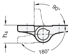
Swiveling range
