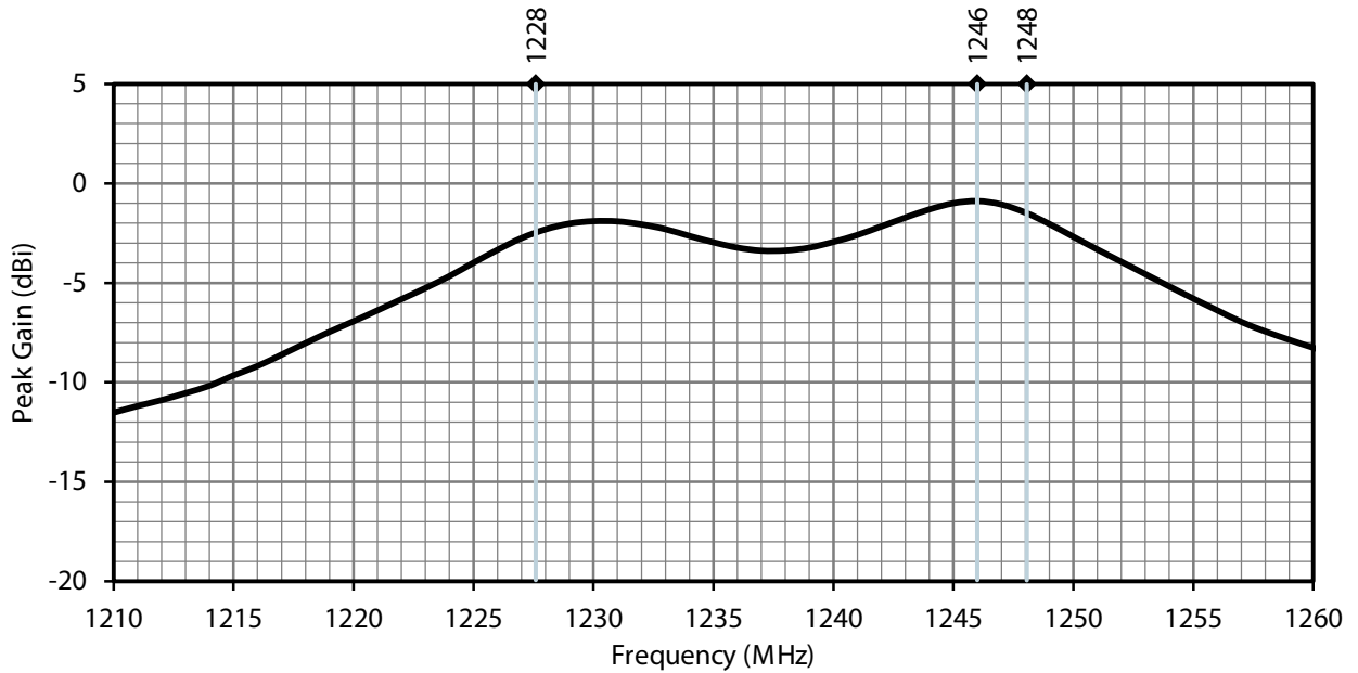
Figure 7. ANT-GNCP-TH25AL12 Peak Gain, L2 Bands
