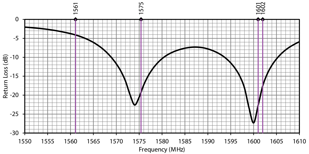
Figure 4. ANT-GNCP-TH25AL12 Return Loss, L1 Bands
