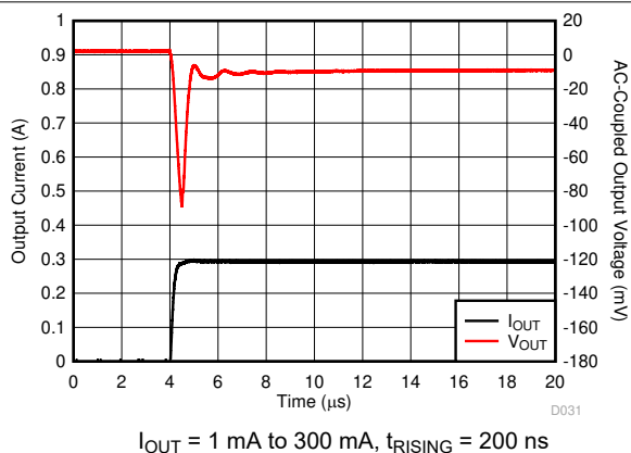
Figure 6-53. Load Transient
