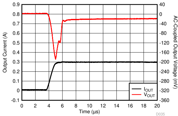
I_{OUT} = 0\text{ mA to } 300\text{ mA} , t_{RISING} = 1\text{ }\mu\text{s}
