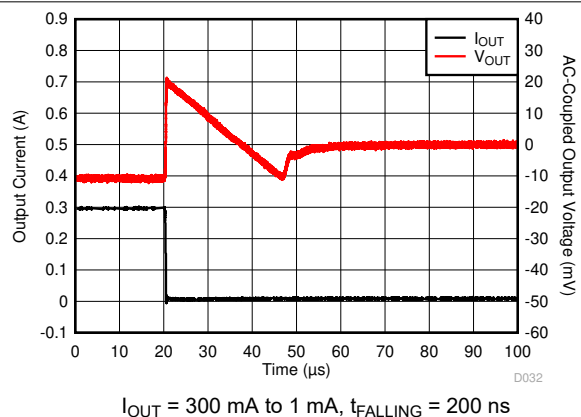
Figure 6-54. Load Transient
