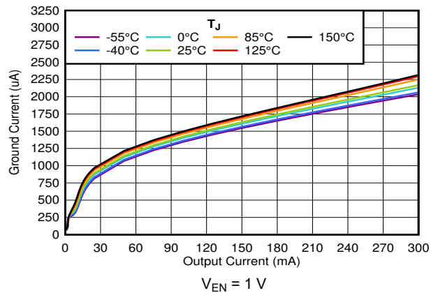
Figure 6-38. I_{GND} vs I_{OUT}
