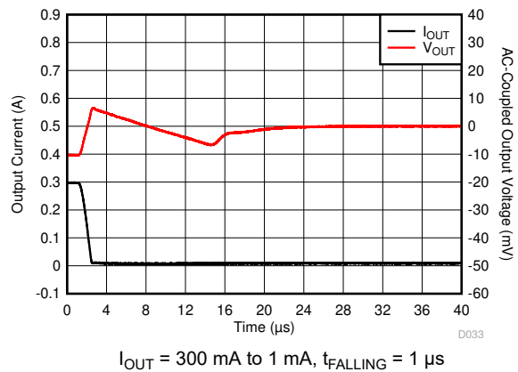
Figure 6-52. Load Transient
