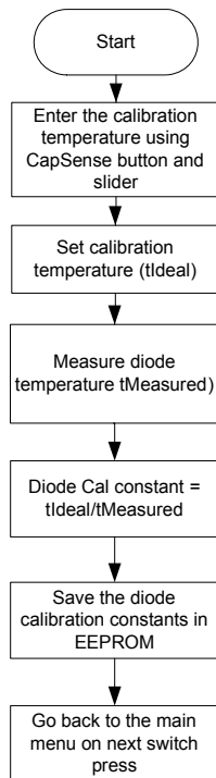
Figure 5-13. Diode Calibration
