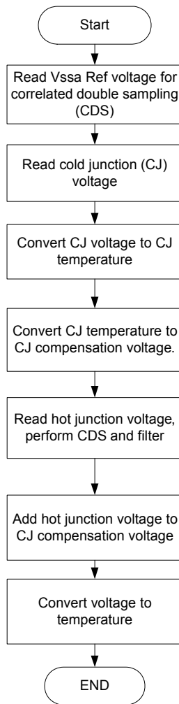
Figure 5-8. Thermocouple Flowchart
