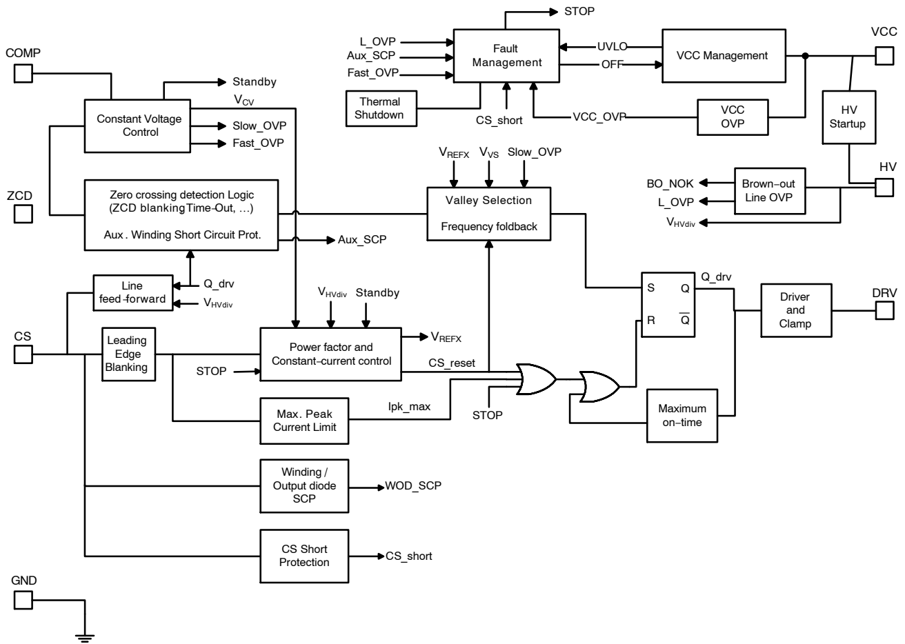
Figure 2. Internal Circuit Architecture NCL30488
