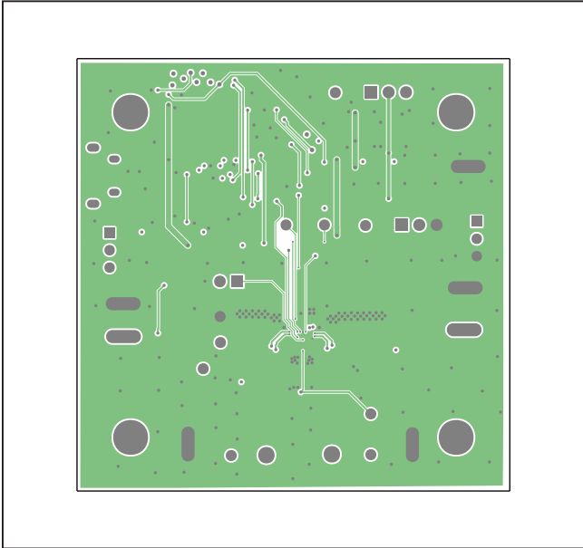
MAX77950 EV Kit PCB Layout—Internal Layer 3
