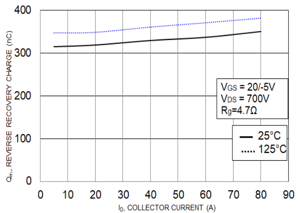
Figure 26. Typical Reverse Recovery Charge vs. I_D
