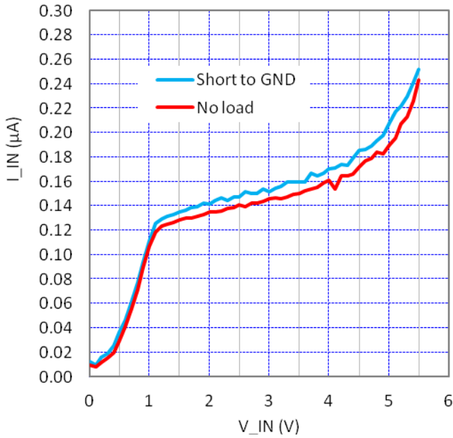
Figure 8. Standby (µA) and Leakage Current (µA) vs. Vin (V)
