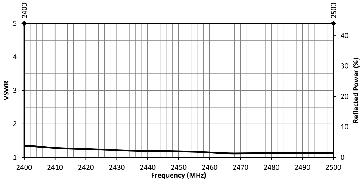
Figure 3. ANT-2.4-MSA-TH1 Antenna VSWR
