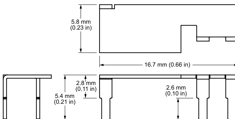
Figure 1. ANT-2.4-MSA-TH1 Antenna Dimensions
