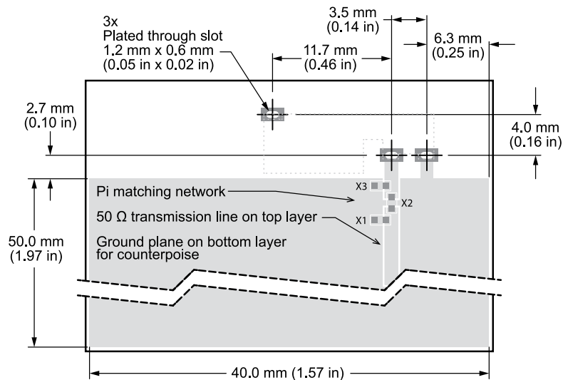
Figure 10. ANT-2.4-MSA-TH1 Recommended Layout
