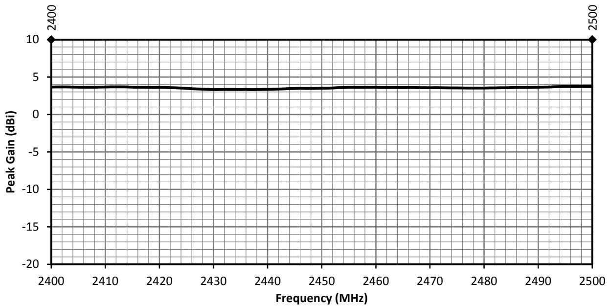
Figure 5. ANT-2.4-MSA-TH1 Antenna Peak Gain
