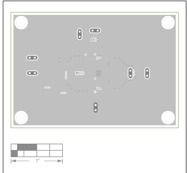
MAX17634A EV Kit—Layer2 GND
