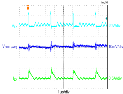
CONDITIONS: DCM MODE, 50mA LOAD
