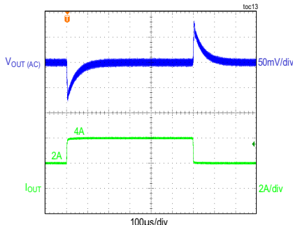
CONDITIONS: PWM/PPM/DCM MODE
