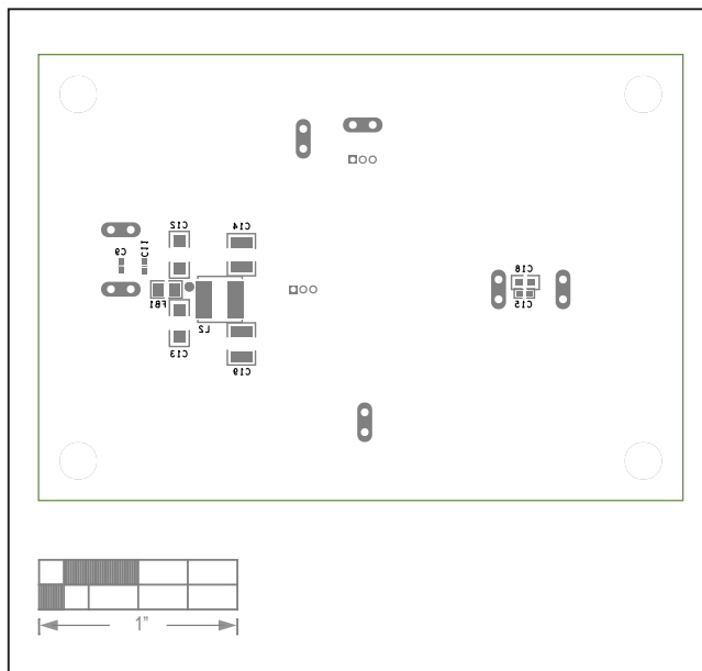
MAX17634A EV Kit—Bottom Silkscreen
