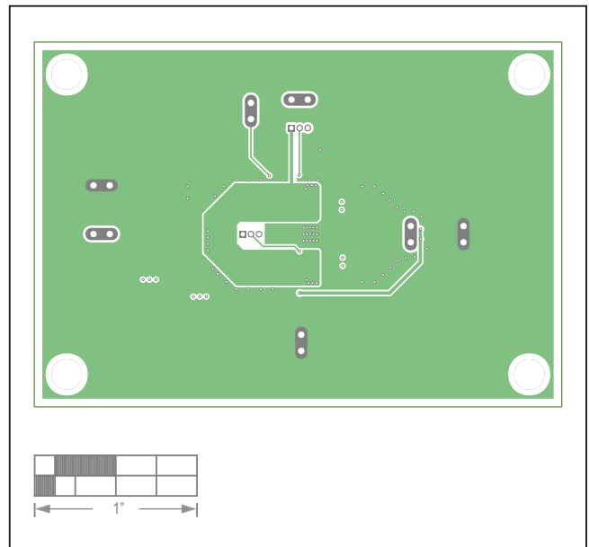
MAX17634A EV Kit—Layer3 GND
