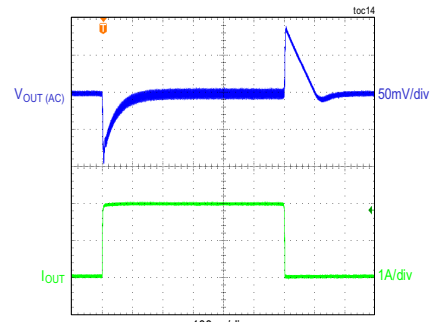
CONDITIONS: DCM MODE
