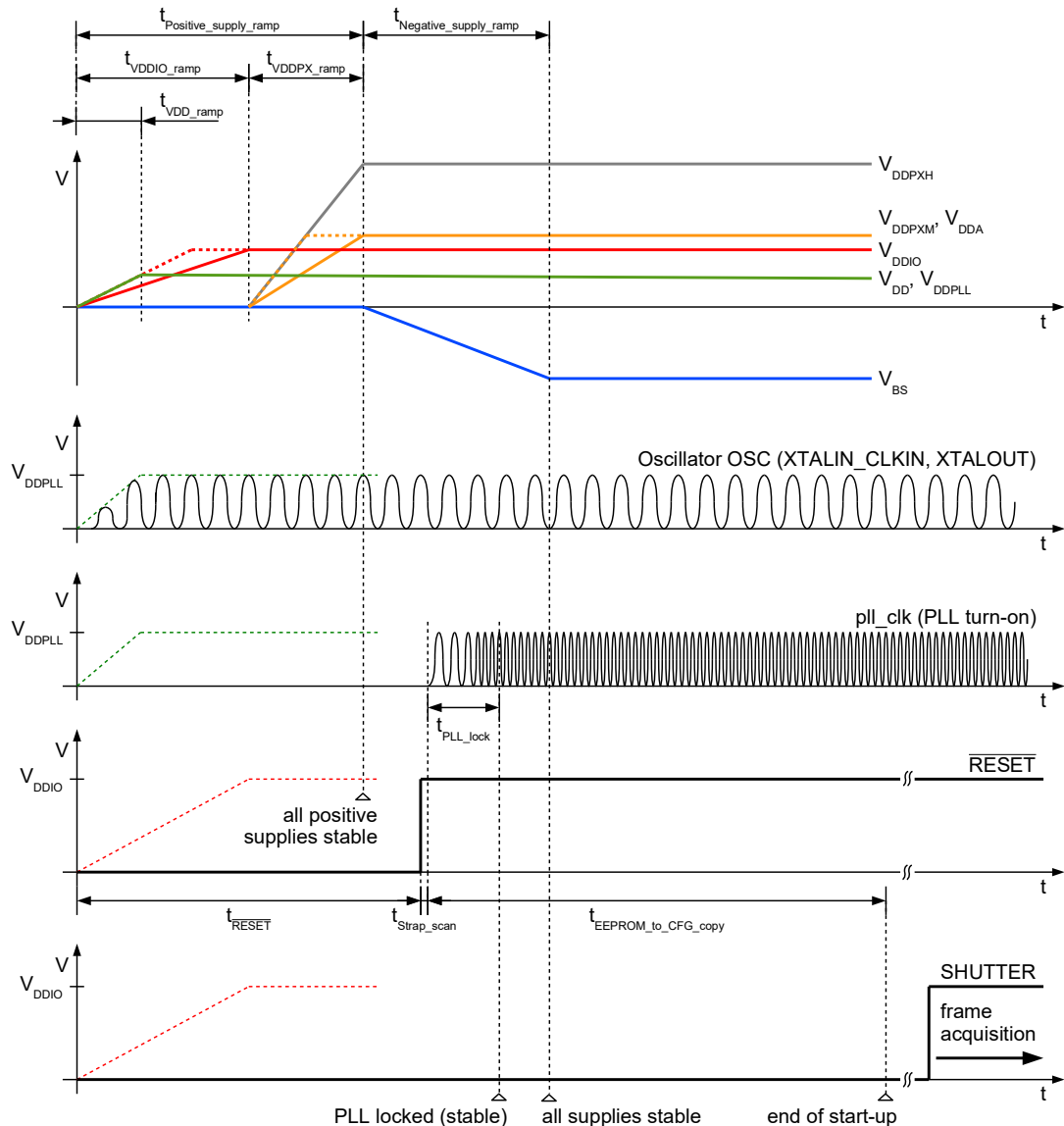
Figure 21: Power-up and reset sequence
