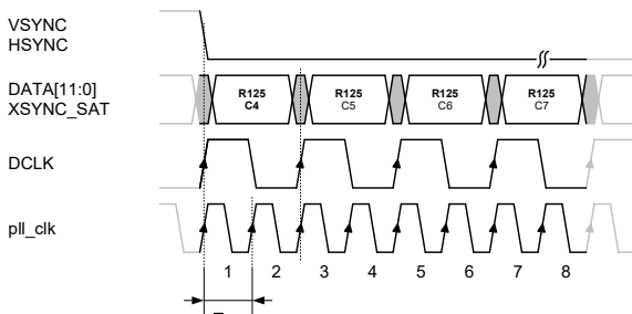
TCMI detailed bus timing: DCLK=48MHz ( pll\_clk / 2 )
