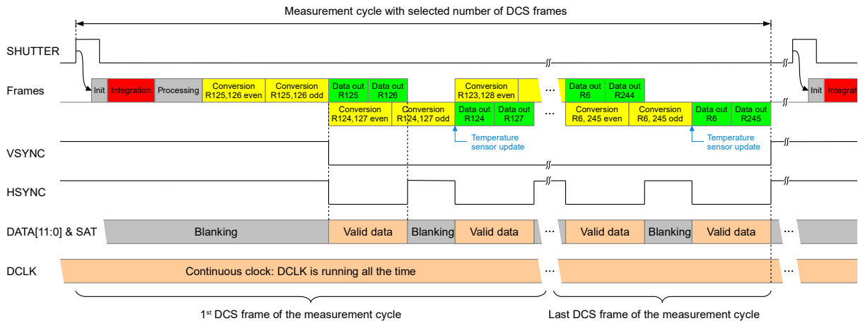
Figure 26: Continuous clock mode
