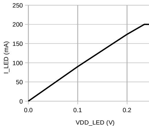
Figure 18: Output characteristic I LED versus V DDLED . Refer for maximum values of V DDLED and I LED to 1 and 2
