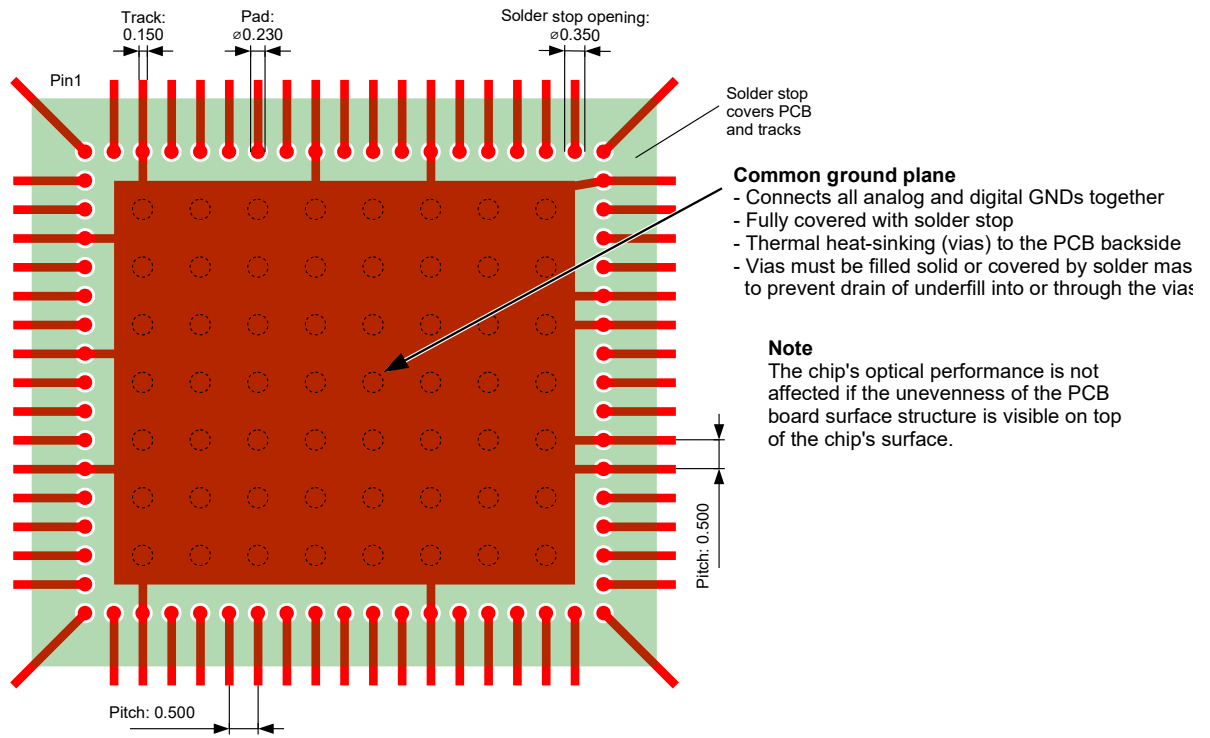
Figure 13: Recommended PCB layout (all measures in mm)
