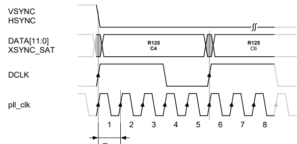
TCMI detailed bus timing: DCLK=19.2MHz ( pll\_clk / 5 )
