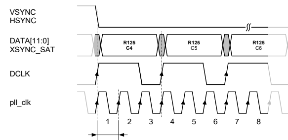
TCMI detailed bus timing: DCLK=32MHz ( pll\_clk / 3 )
