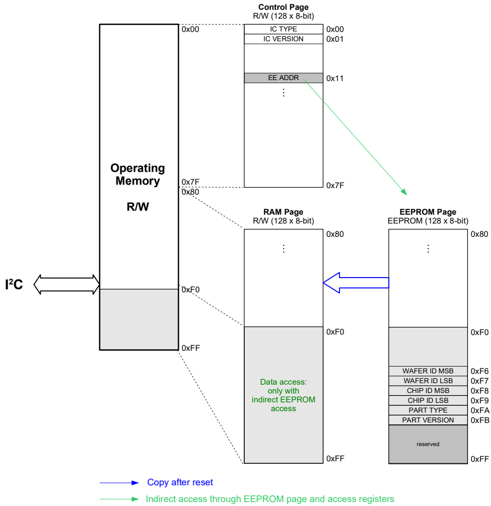
Figure 58: Memory map
