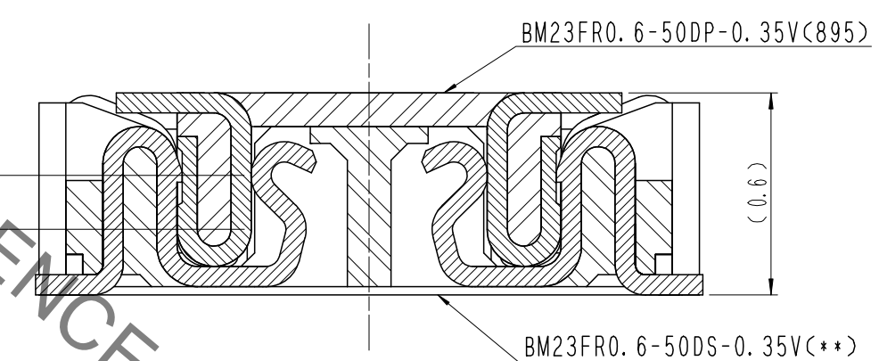
ENGAGEMENT FIGURE (50:1)
