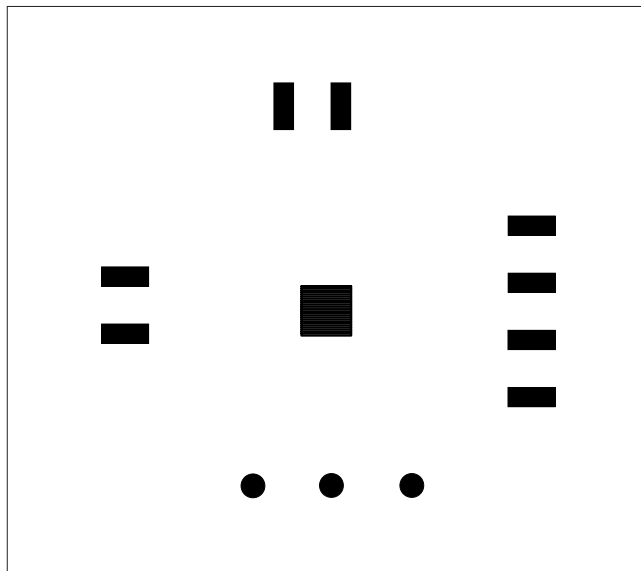
Figure 9. MAX9994 EV Kit PC Board Layout— Bottom Soldermask
