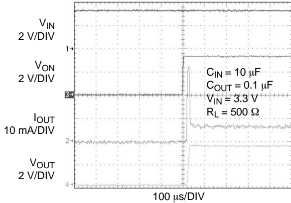
Figure 18. t_{ON} Response
