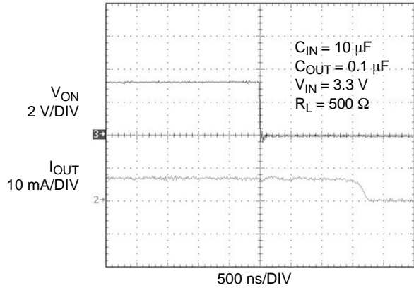
Figure 19. t_{OFF} Response
