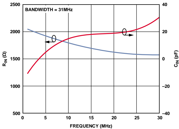
Figure 37. Input Impedance vs. Frequency (Bandwidth Setting = 31 MHz)
