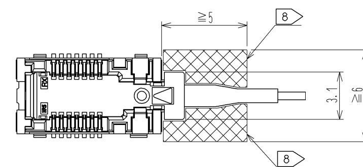
Dimensions of engaged connector (Scale:FREE)
