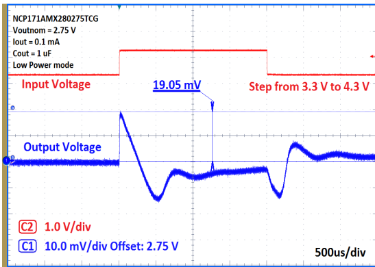
Figure 66. Line Transient Response in Low Power Mode
