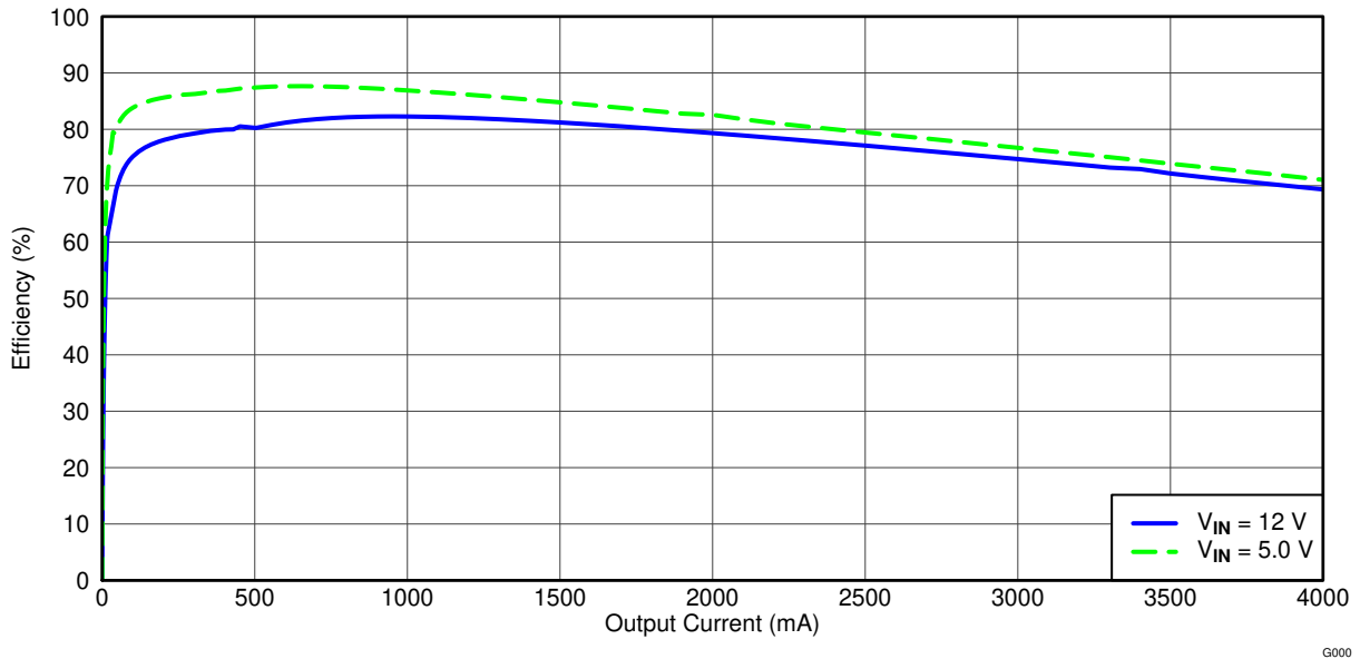
Figure 4-1. TPS54428EVM-052 Efficiency
