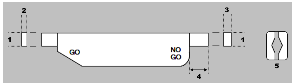
Figure 7: Recommended plug gage design for insulation barrel section of crimping chamber
