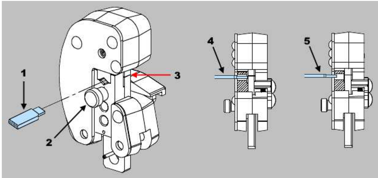
Figure 9: Inspecting the insulation barrel crimping dies
