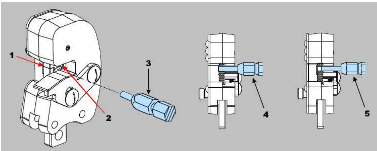
Figure 8: Inspecting the wire barrel crimping dies
