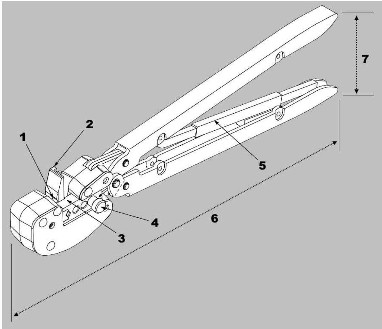
Figure 1: PIDG PEEK STRATO-THERM terminal crimping tool
