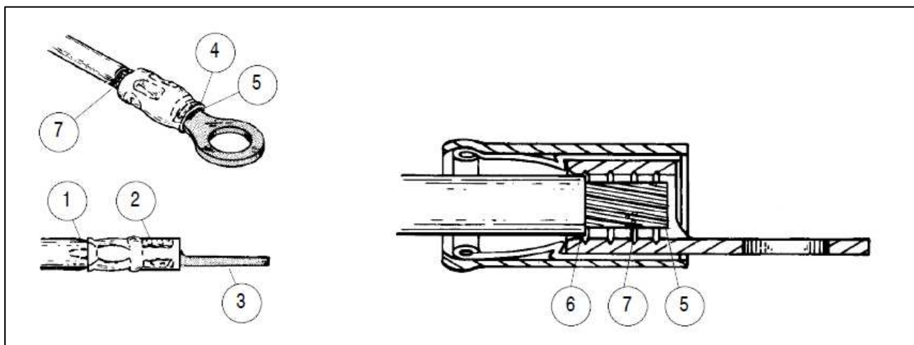
Figure 4: Features of a poor crimp
