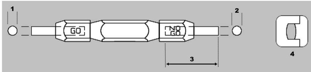
Figure 6: Recommended plug gage design for wire barrel section of crimping chamber
