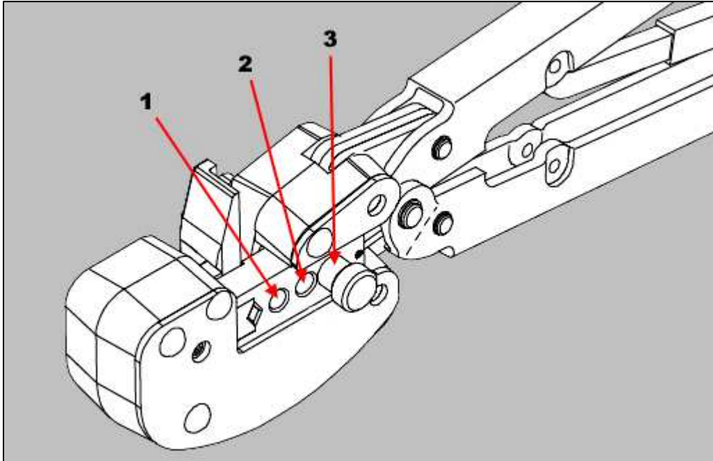
Figure 5: Insulation crimp adjustment pin
