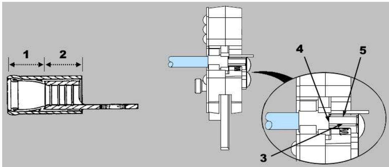
Figure 2: Crimping
