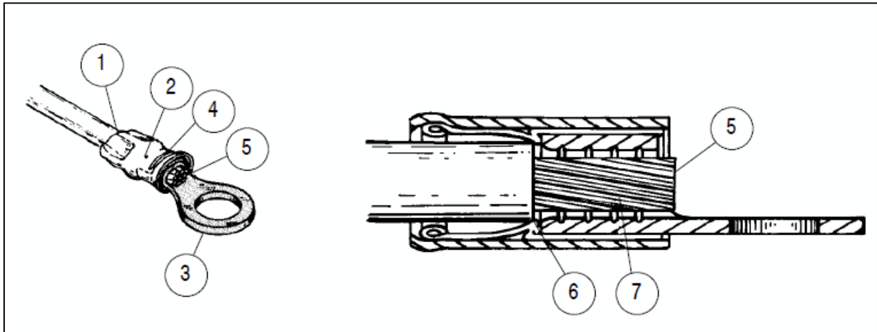
Figure 3: Features of a good crimp
