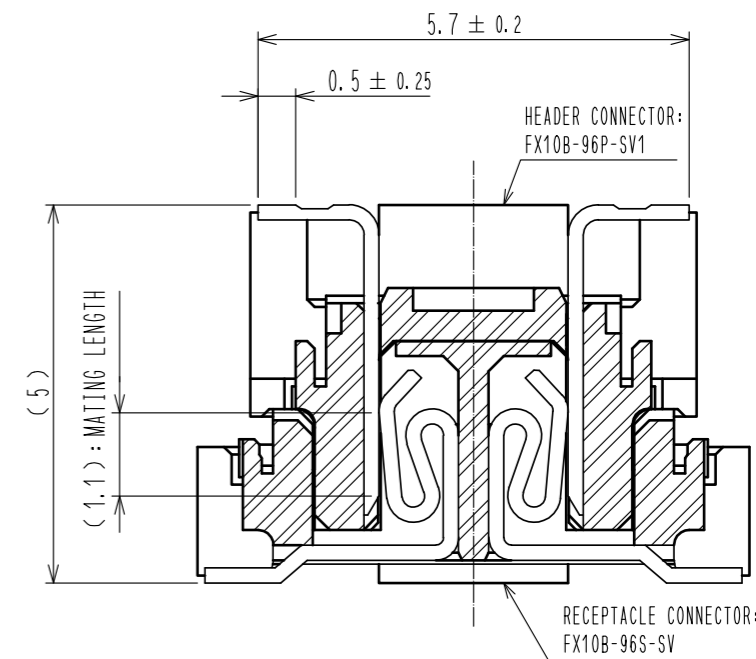
CROSS CUT SECTION (10:1)
