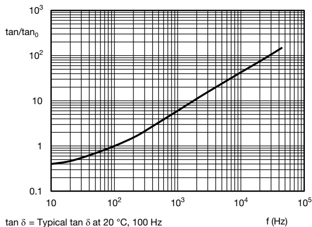
Fig. 9 - Typical multiplier of dissipation factor (tan δ) as a function of frequency
