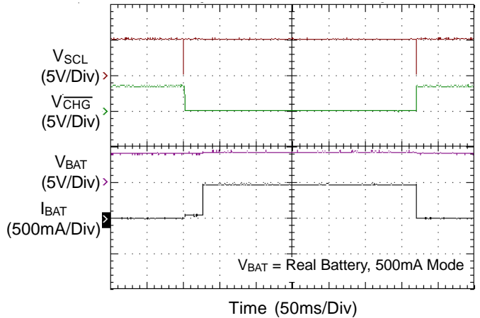
Charge on/Off Control by I 2 C
