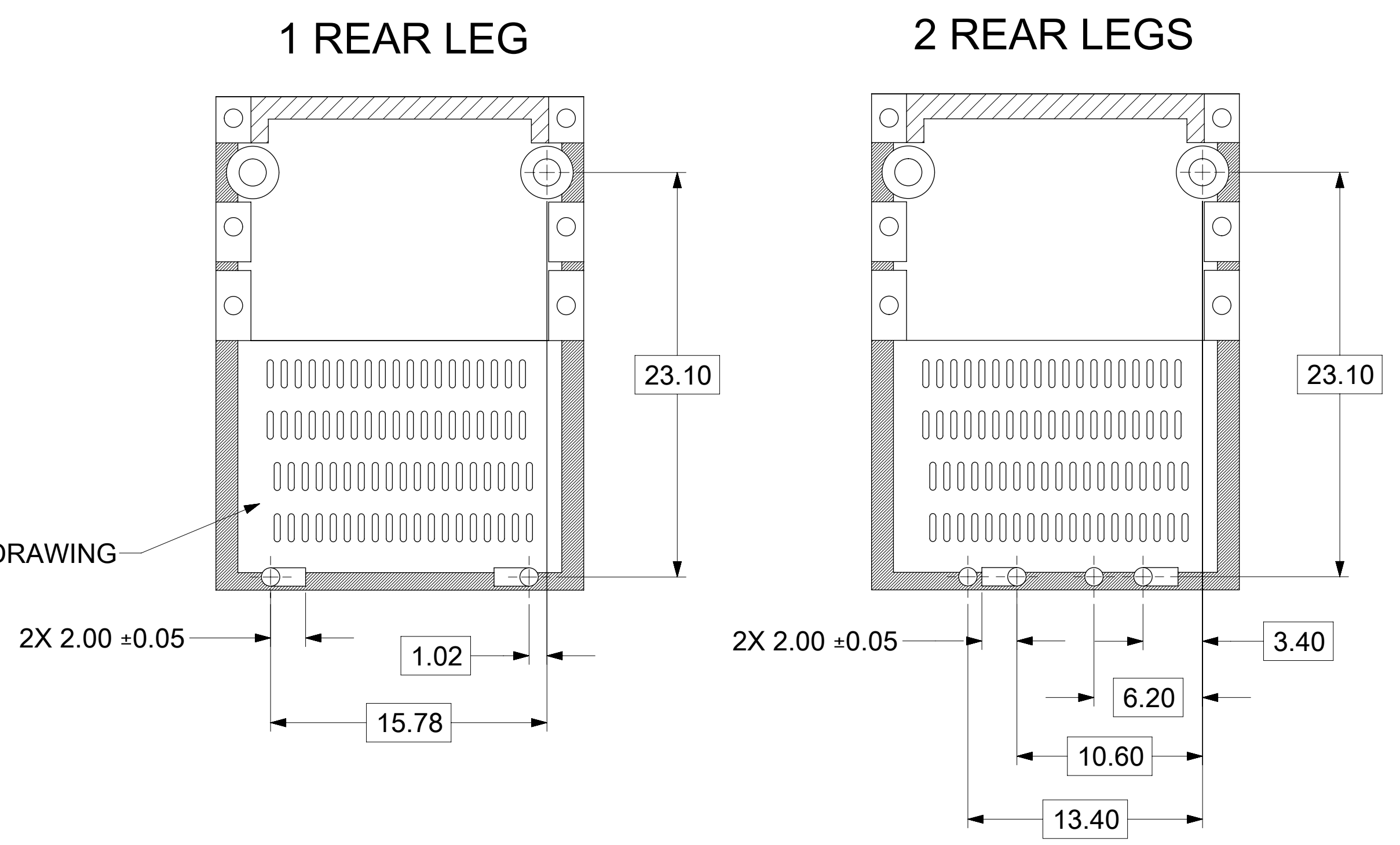
PARTIAL 2 SCALE 4:1
