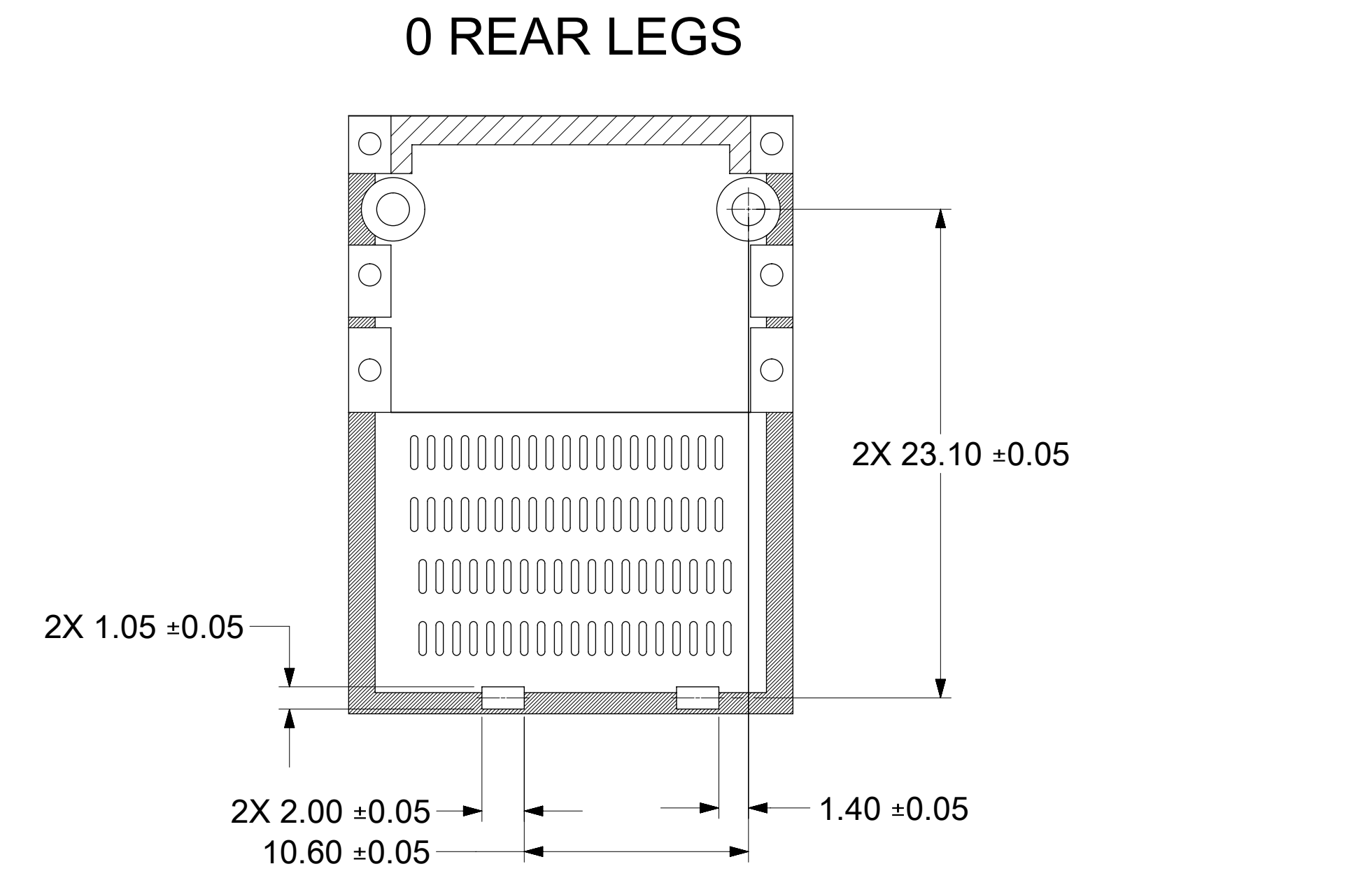
PARTIAL 1 SCALE 4:1
