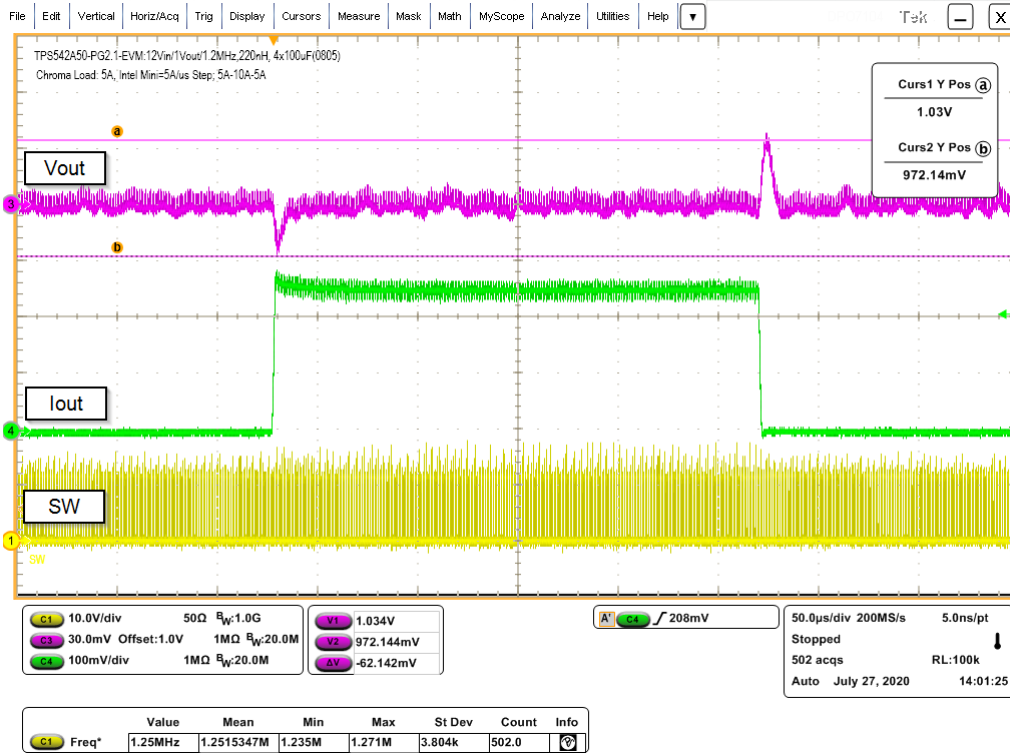
Figure 4-6. Transient Response - 5-A to 10-A to 5-A Load at 5 A/ \mu s, \Delta Vout = 62.1 mV, fsw = 1200 kHz, FCCM
