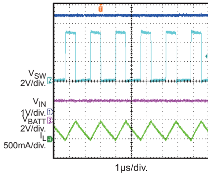
TC Charge Steady State V_{BATT\_FULL} = 4.2V , V_{BATT} = 2V , F_{SW} = 600kHz
