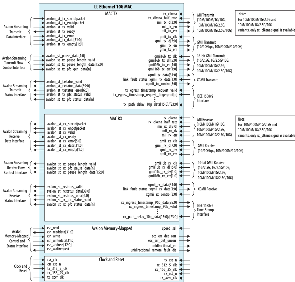
Figure 9. Interface Signals
