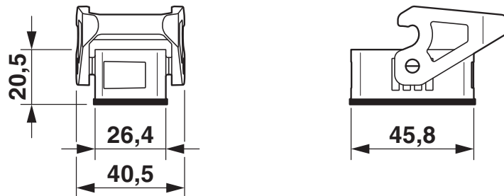
Dimensional drawing
