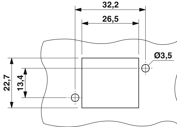
Dimensional drawing
