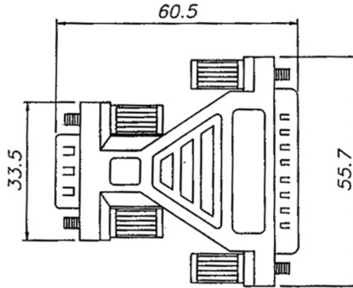
P1 MOLDED
