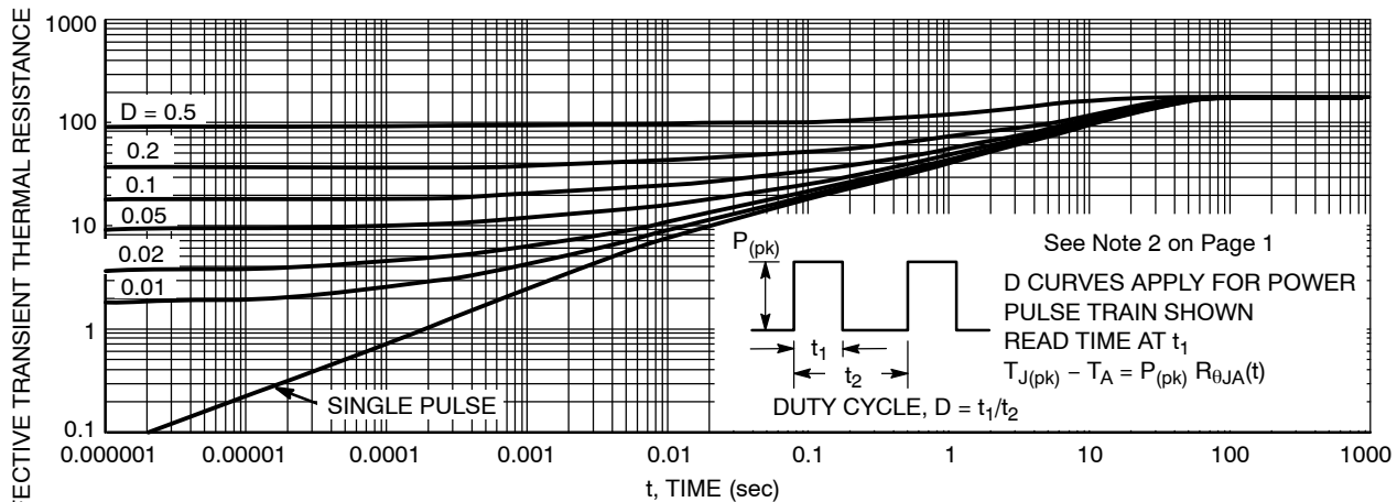
Figure 12. Thermal Response
