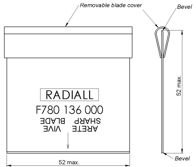
Dimension in mm [inch]
