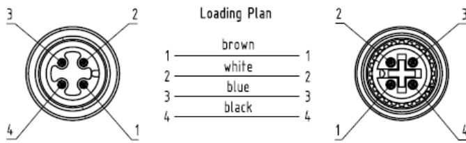
Male and Female 4-pole
