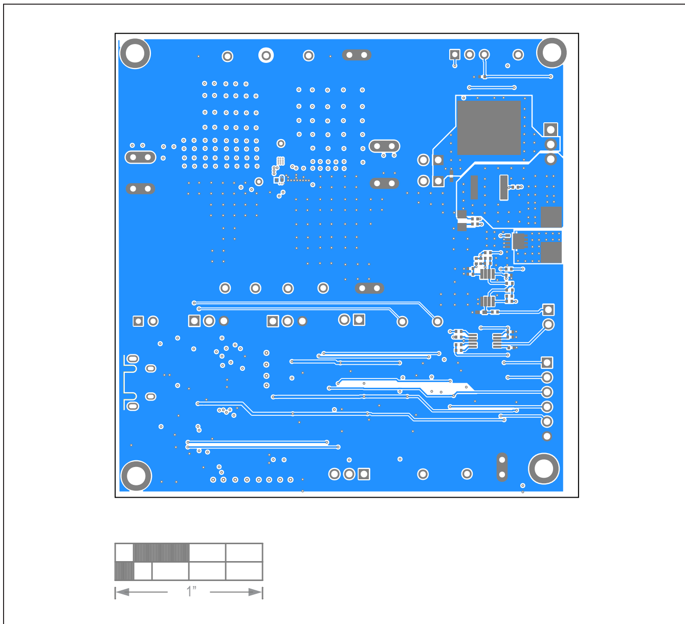
MAX77533 EV Kit PCB Layout—Bottom Layer
