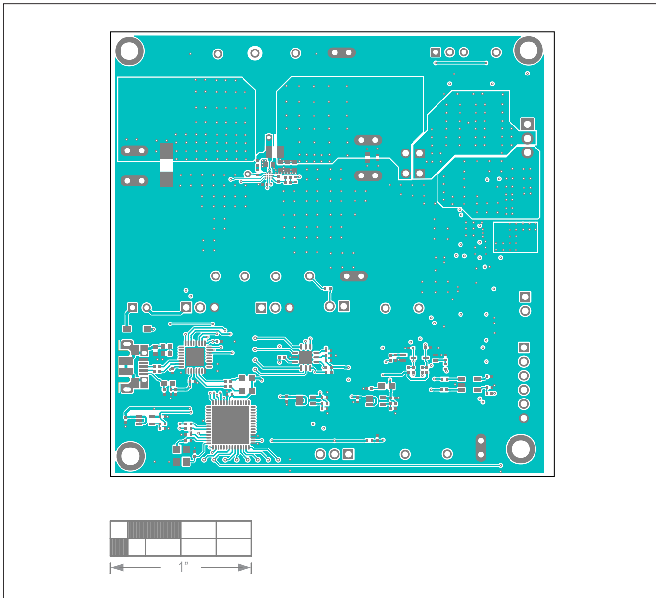
MAX77533 EV Kit PCB Layout—Top Layer
