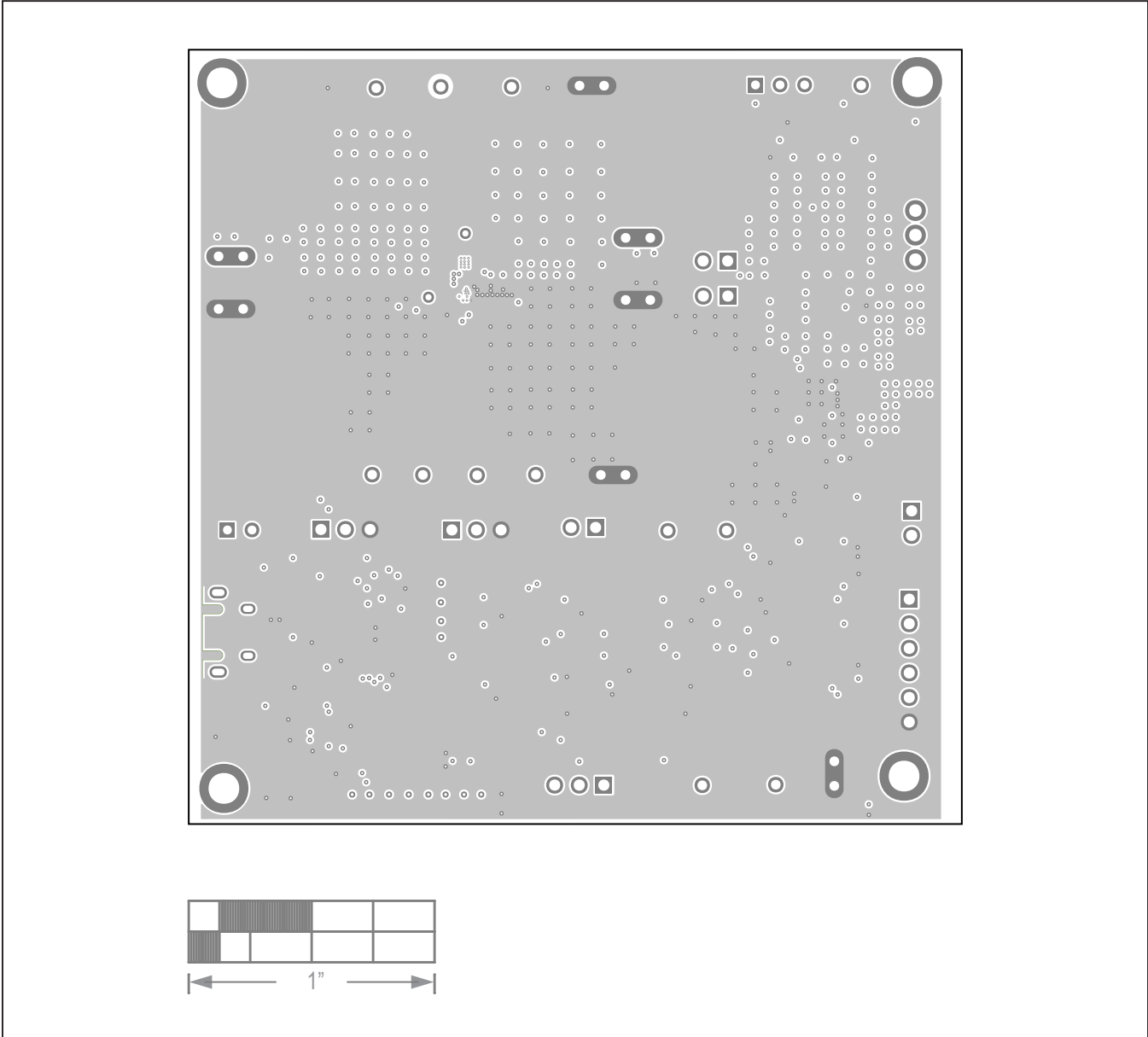
MAX77533 EV Kit PCB Layout—Internal Layer 2
